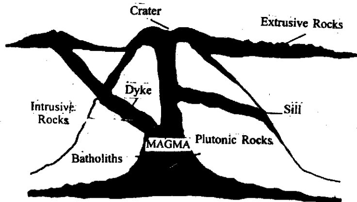
Fig. 7.2 Igneous Rocks
