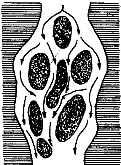
Fig 11.6 Braided Stream
