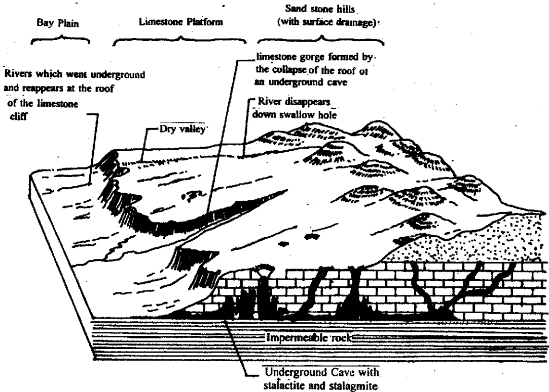
Fig. 11.16 Limestone Landscape
