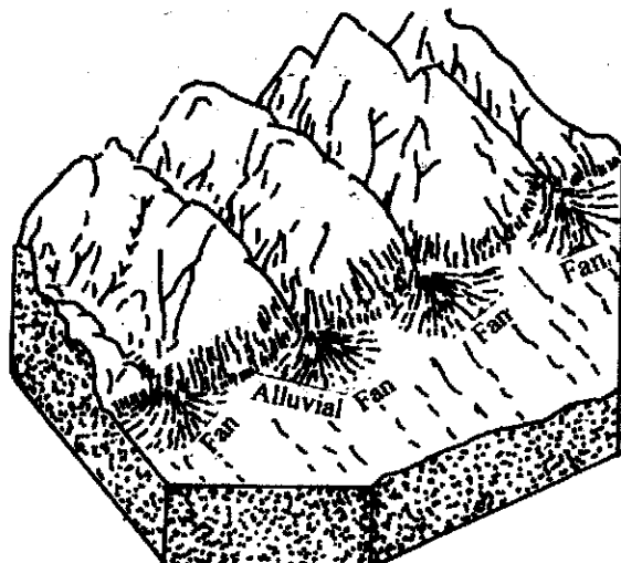
Fig. 11.5 Alluvial Fans
