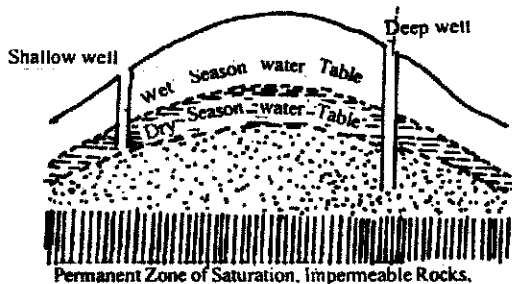
Fig. 11.10 Water Table
